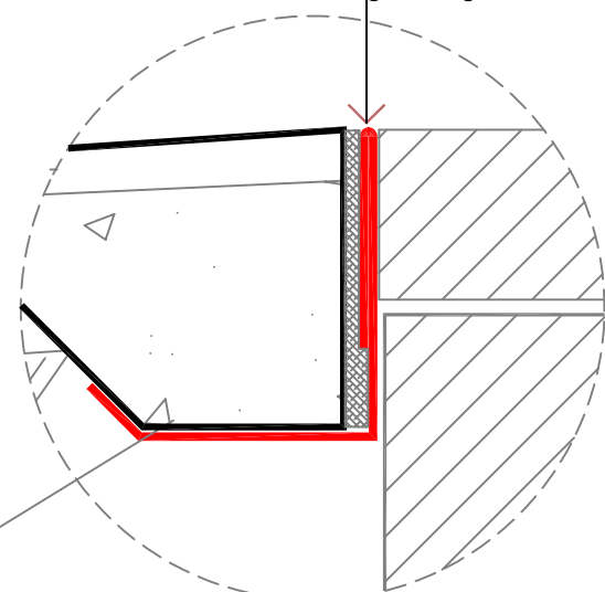
section detail 2
