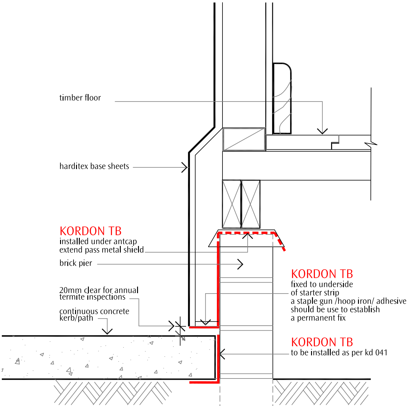
section detail 1 bearers & joist
