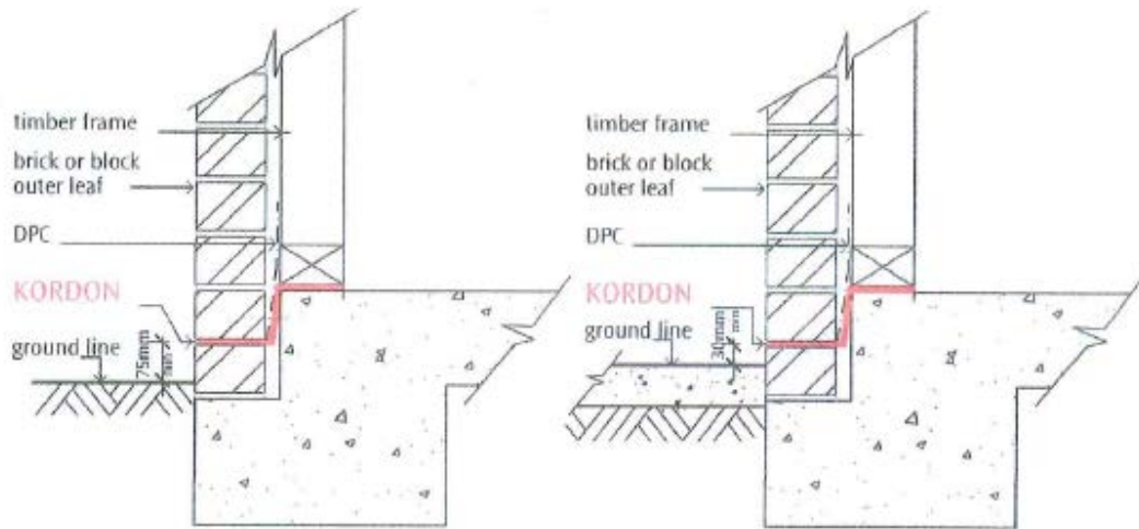
section detail 1
