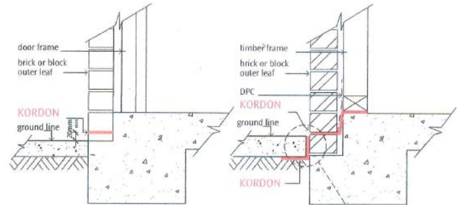
section detail 3
